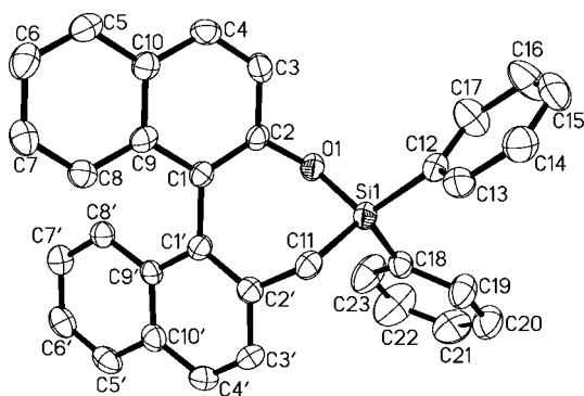
Figure 5. Molecular structure of (P)-(R ax )-9 [derived from (S ax )-binol ]. Hydrogen atoms omitted for clarity; displacement ellipsoids drawn at 50% probability level. Selected inter atomic distances [Å] and angles [°]: Si(1)–O(1) 1.667(2), Si(1)–C(11) 1.866(3), O(1)–Si(1)–C(11) 104.45(10), C(18)–Si(1)–C(12) 110.37(10); torsion angle C(2)–C(1)–C(1')–C(2') 57.9(3).
