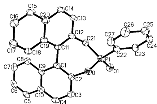
Figure 7. Molecular structure of (P)-(S ax ,R P )-11a derived from (S ax )-binol . Hydrogen atoms omitted for clarity; displacement ellipsoids drawn at 50% probability level. Selected inter atomic distances [Å] and angles [°]: P(1)–O 1.691(2), P(1)–O(1) 1.4732(12), P(1)–C(21) 1.813(2), P(1)–C(22) 1.793(2), C(21)–P(1)–O 102.45(7), C(22)–P(1)–O(1) 113.45(8); torsion angle C(2)–C(1)–C(11)–C(12) 54.8(2).
