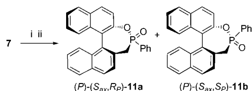
Scheme 5. Preparation of phosphane oxide 11a . Reagents and conditions: (i): a) 7 (1 equiv.), n BuLi (3 equiv.), TMEDA (3 equiv.), \text{Et}_2\text{O} , 0 °C, 24 h. [leads to (P)-(S ax ,R P )-11a only]; or b) 7 (1 equiv.), n BuLi (2.5 equiv.), t BuOK (2.5 equiv.), \text{Et}_2\text{O} , –40 °C, 3 h [leads to a 5:6 mixture of (P)-(S ax ,R P )-11a and its S P epimer 11b ] (ii) \text{PhP}(\text{=O})\text{Cl}_2 (2.0 or 1.5 equiv.), –60 °C, 3 h.
