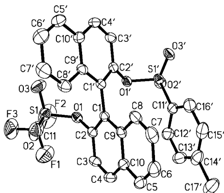
Figure 2. Molecular structure of (M)-(R ax )-5a . Hydrogen atoms omitted for clarity, displacement ellipsoids drawn at 50% probability level. Selected inter atomic distances [Å] and angles [°]: S(1)–O(1) 1.566(2), S(1')–O(1') 1.604(2); torsion angle C(2)–C(1)–C(1')–C(2') –70.2(3).
